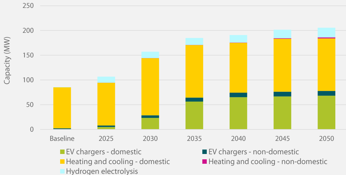
Figure 3 Cumulative disruptive electricity demand capacity in Orkney, Consumer Transformation scenario
