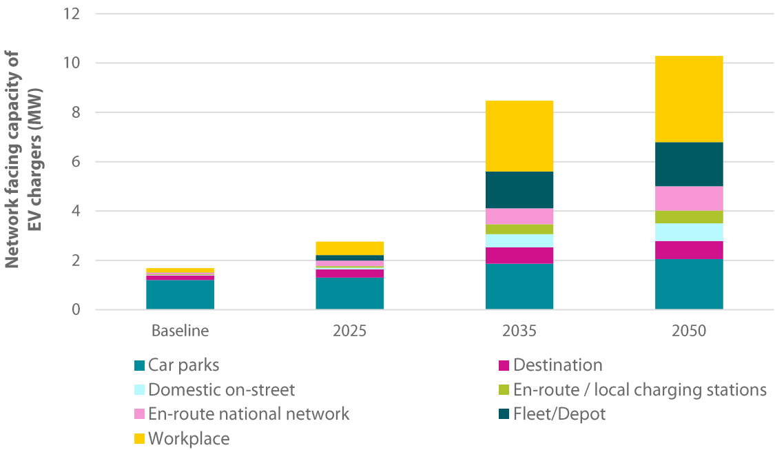
Figure 19 Projected cumulative EV charger capacity in Orkney
