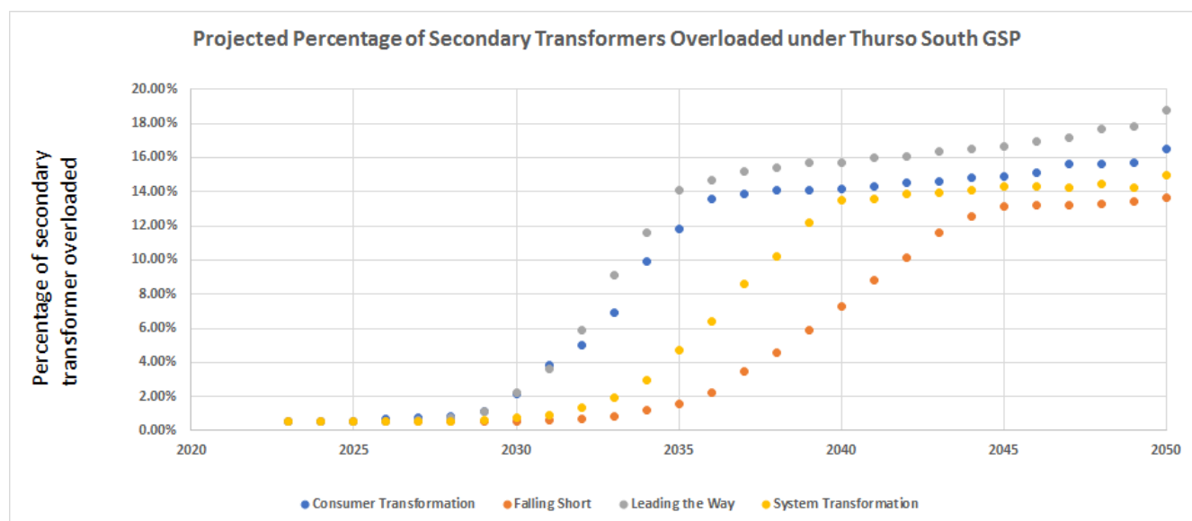
Figure 39 Thurso South Projected Secondary Transformer Loading. Source: SSEN Load Model
