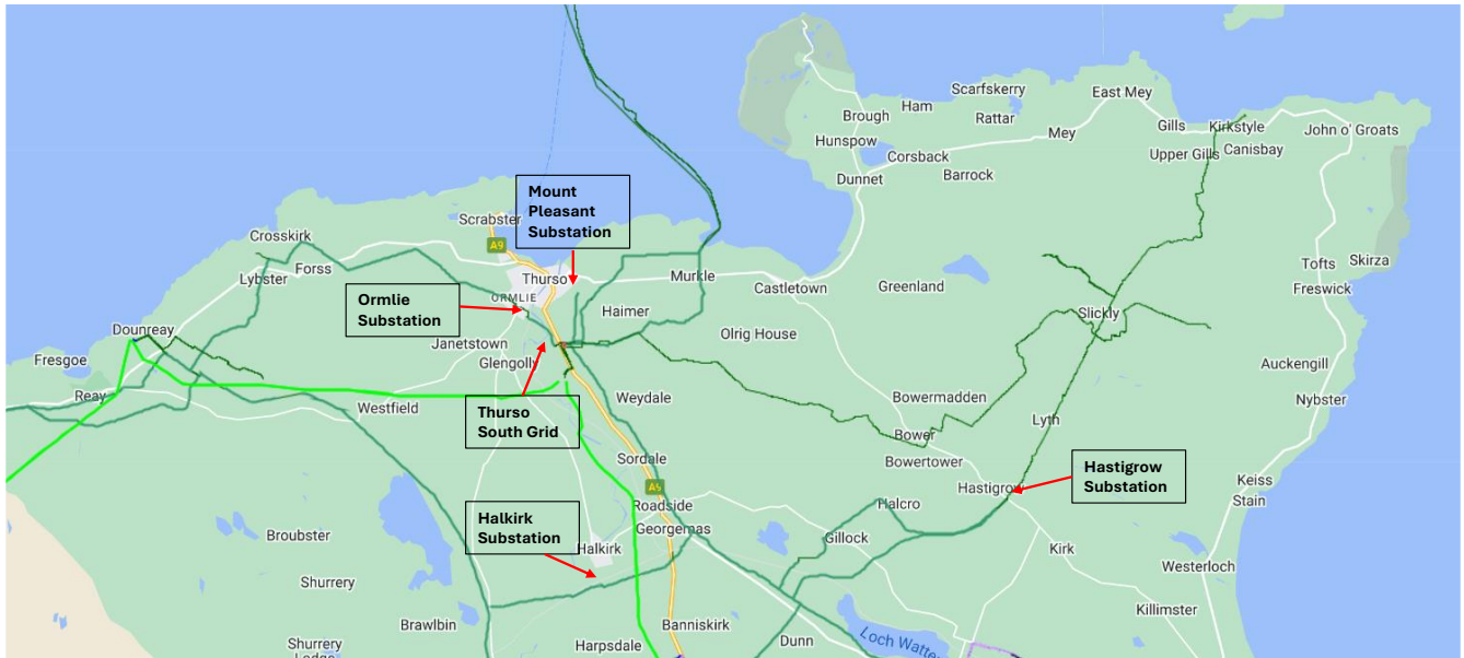
Figure 8 Existing Thurso South Mainland Network Topology
