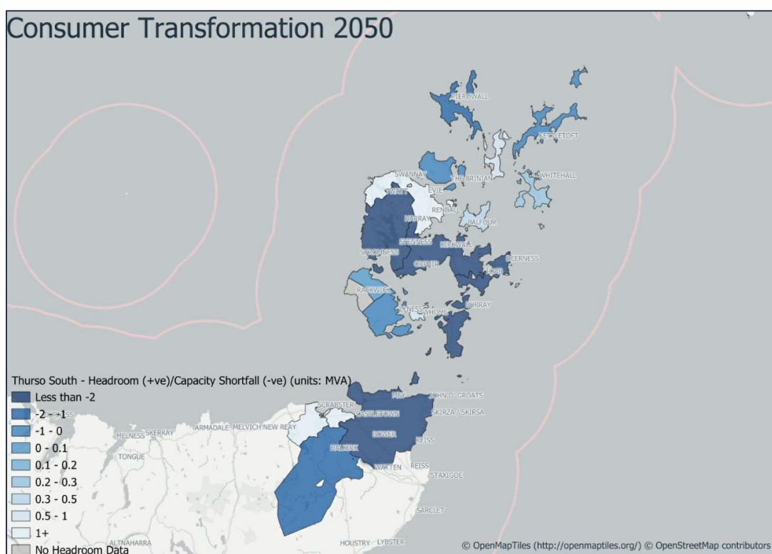
Figure 3 Thurso South GSP 2050 EHV network spatial plan (CT scenario)
