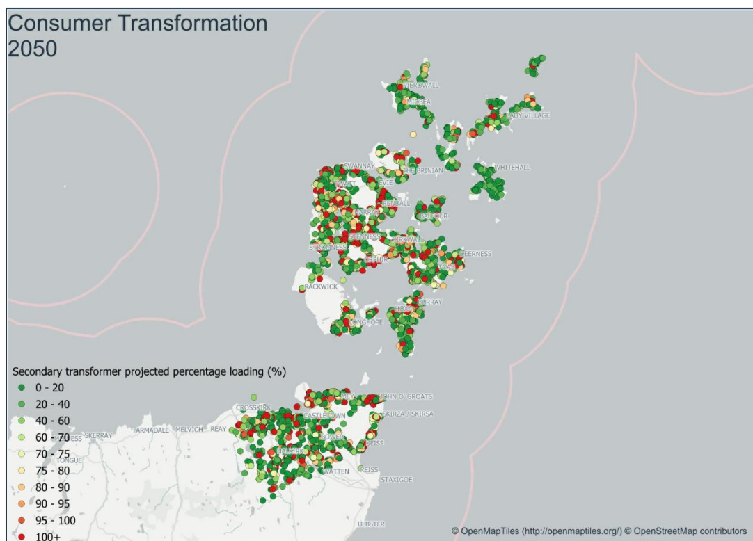
Figure 4 Thurso South GSP 2050 HV/LV network spatial plan.
