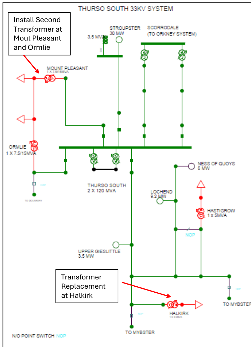
Figure 22 Schematic network with works in progress at Thurso South Mainland
