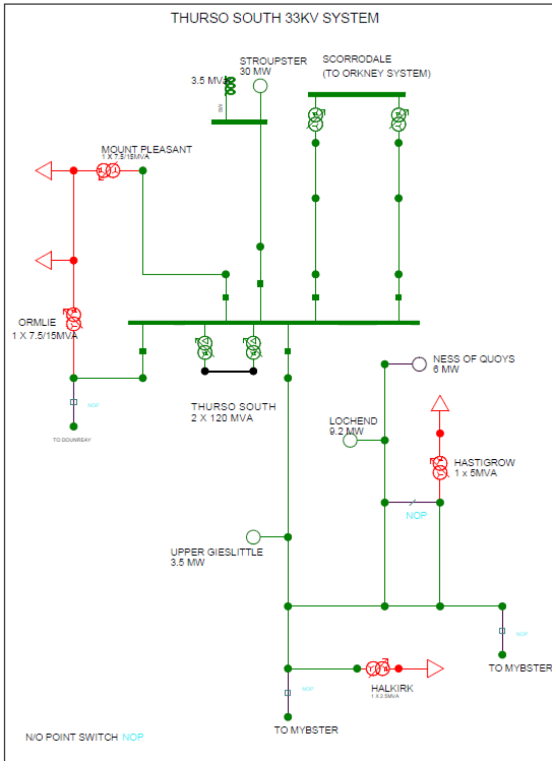
Figure 10 Existing Thurso South 33kV Network
