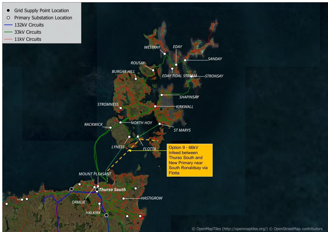
Figure 37 Network schematic with system needs 2041-2050 Option 9.
