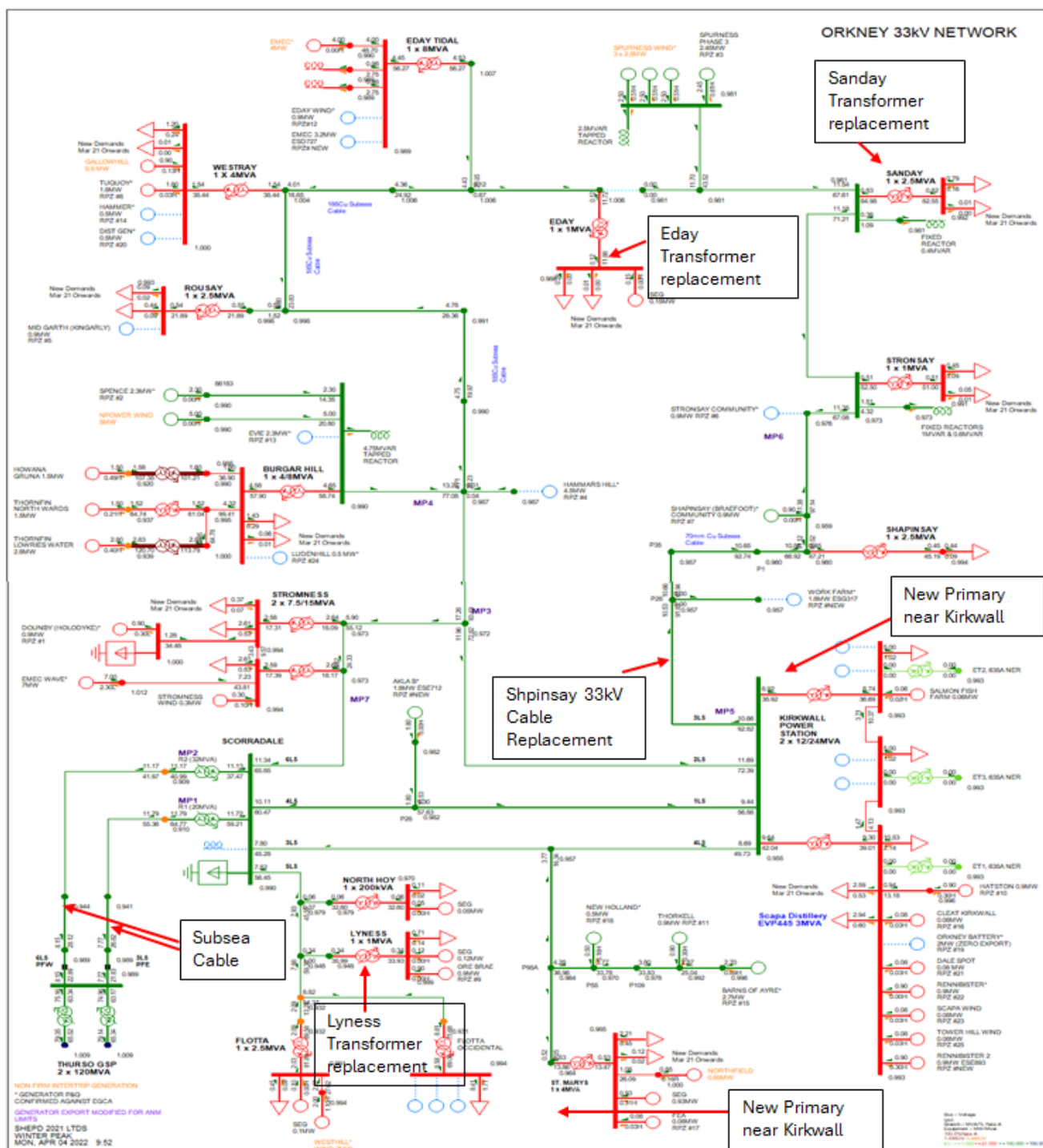
Figure 21 Schematic network with works in progress at Orkney
