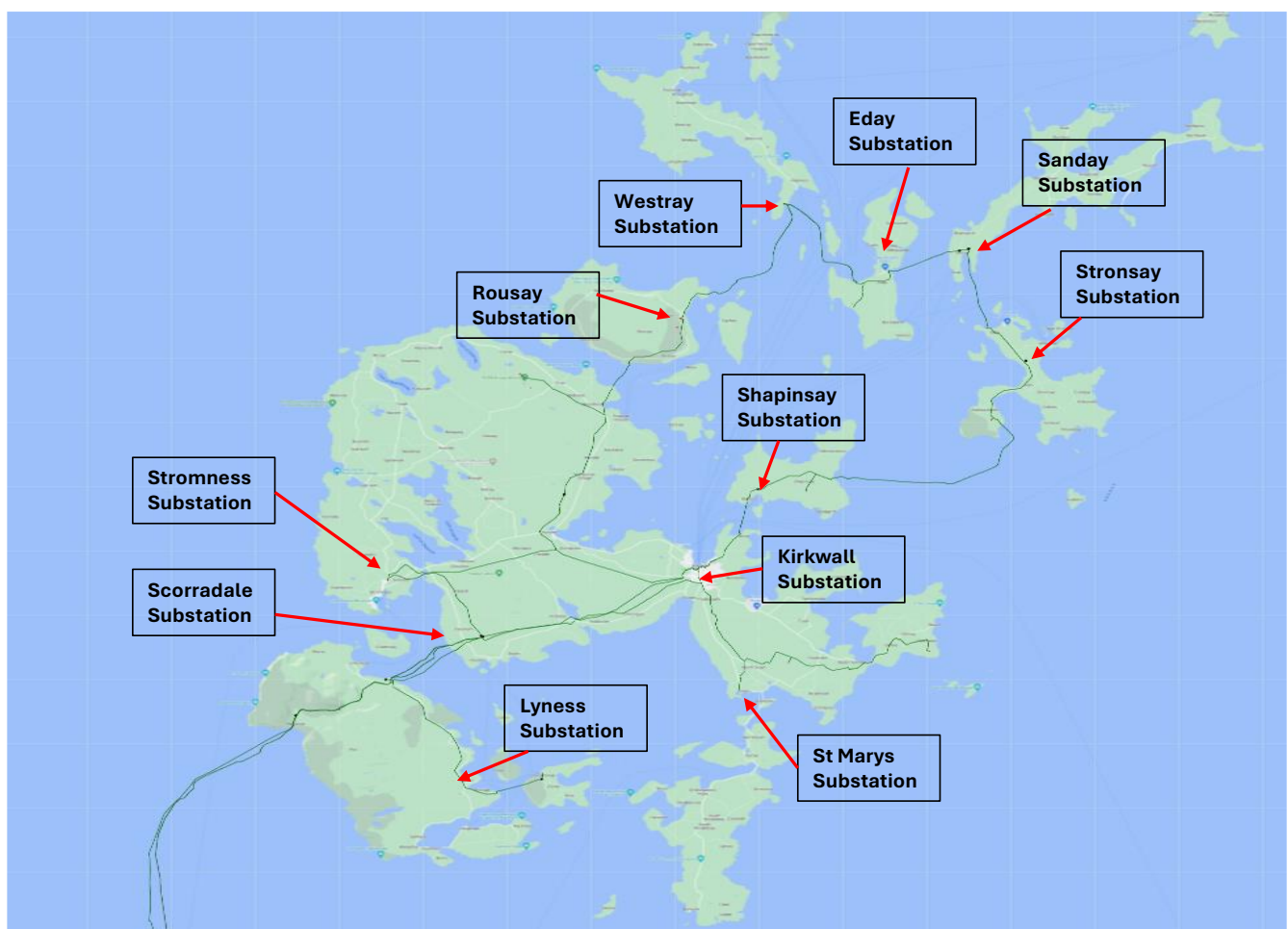
Figure 7 Existing Orkney Network Topology
