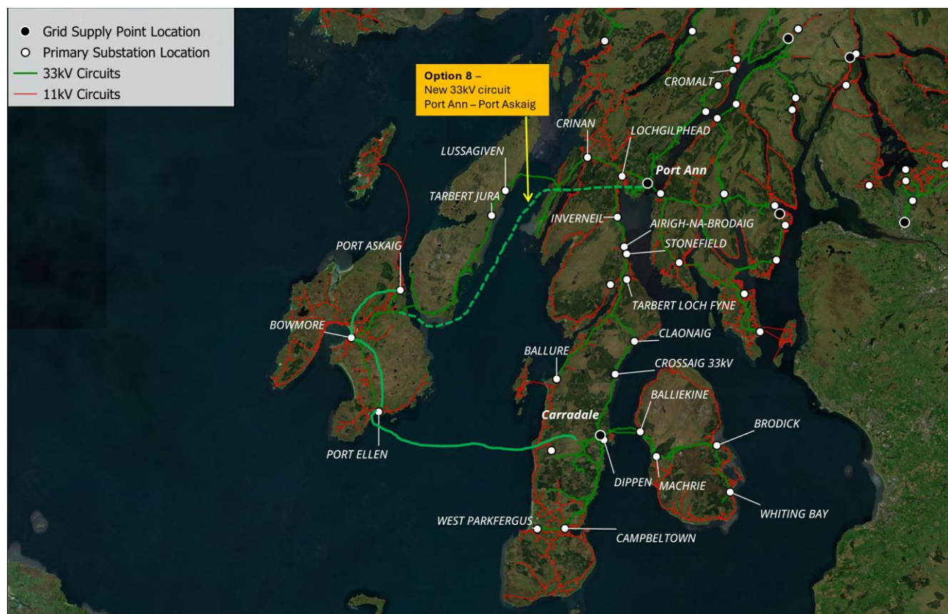
Figure 37 GIS view of network with works in progress and additional reinforcement options by 2040 (Option 8)
