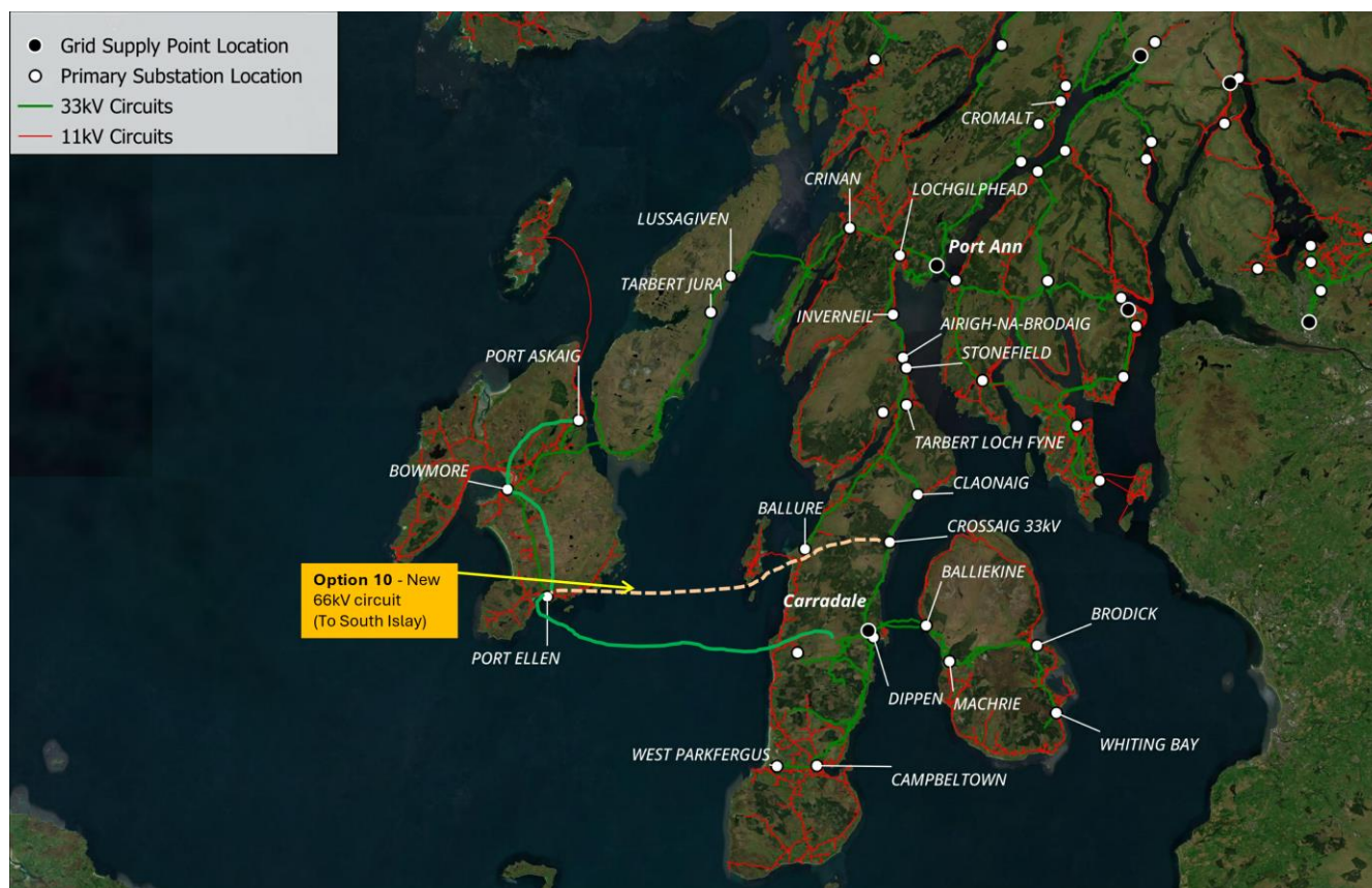
Figure 39 GIS view of network with works in progress and additional reinforcement options by 2040 (Option 10)
