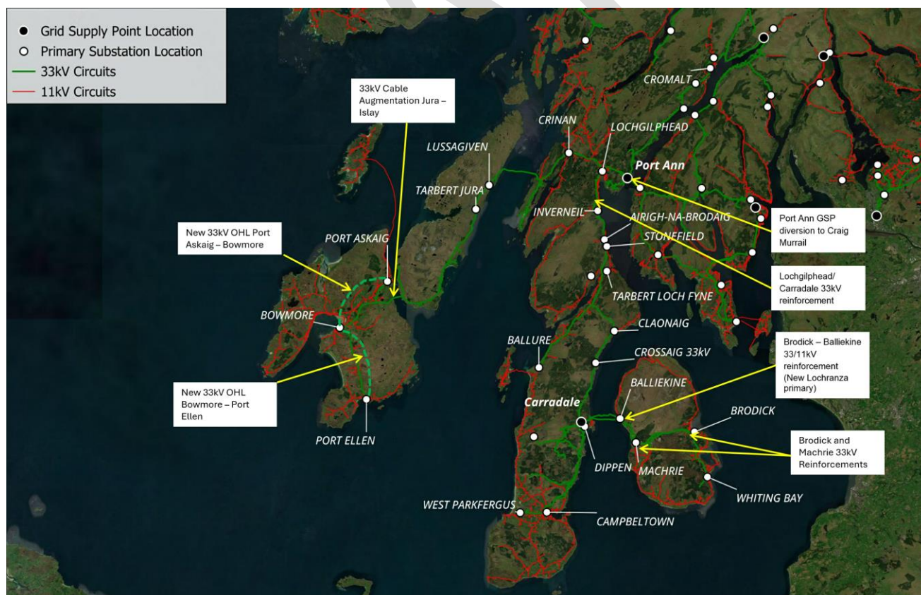
Figure 22 GIS View of Works in Progress and system needs annotated
