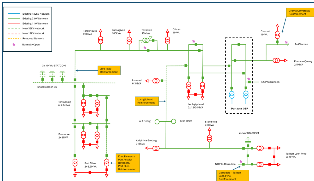
Figure 20 Future Network Development around Port Ann GSP
