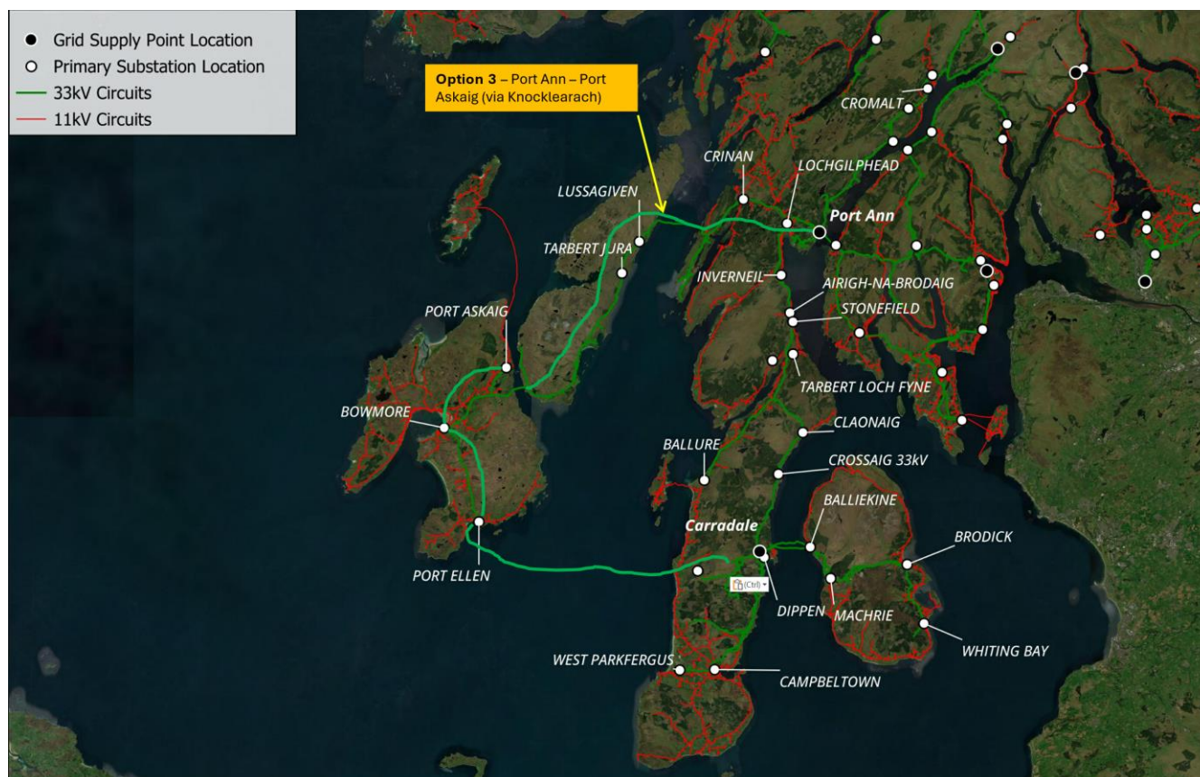
Figure 32 GIS view of network with works in progress and additional reinforcement options by 2040 (Option 3)
