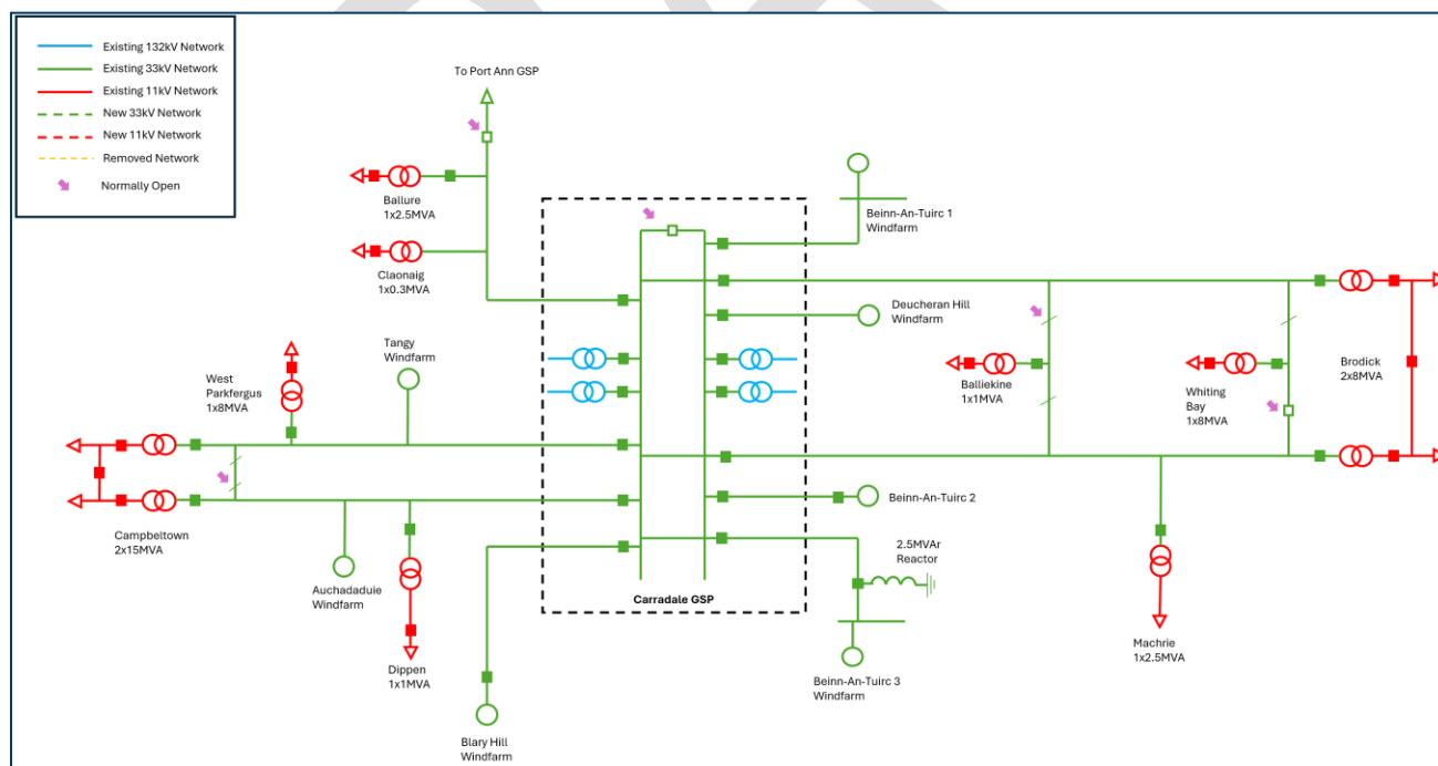
Figure 9 Carradale GSP network schematic – current running arrangement – transformer nameplate ratings
