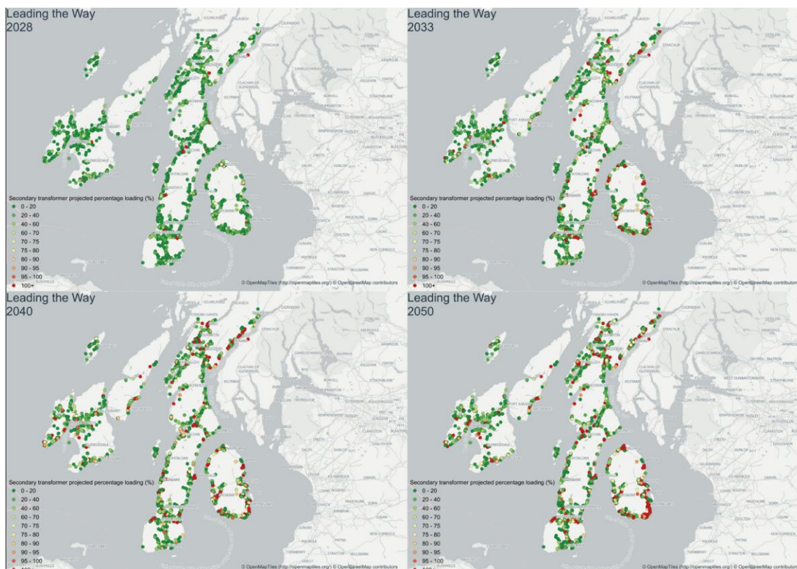
Figure 28 Port Ann and Carradale GSPs HV/LV LW spatial plans for 2028, 2033, 2040, and 2050
