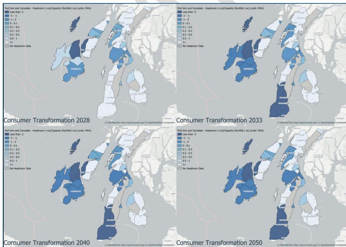
Figure 23 Port Ann and Carradale GSPs EHV spatial plans for CT 2028, 2033, 2040, and 2050
