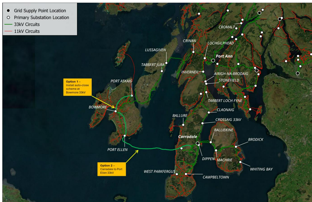
Figure 31 GIS view of network with works in progress and additional reinforcement options by 2028(Options 1 & 2)
