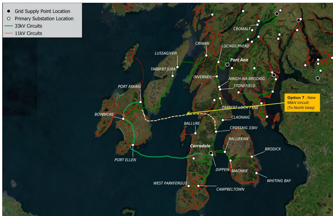
Figure 36 GIS view of network with works in progress and additional reinforcement options by 2040 (Option 7)
