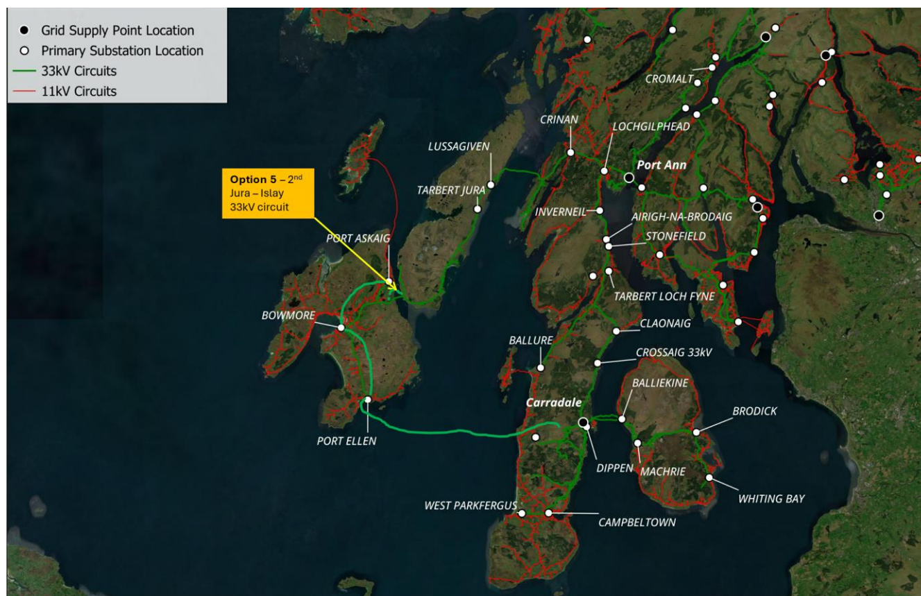
Figure 34 GIS view of network with works in progress and additional reinforcement options by 2040 (Option 5)
