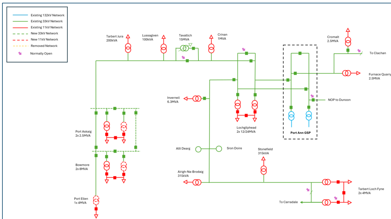
Figure 8 Port Ann GSP network schematic – current running arrangement – transformer nameplate ratings
