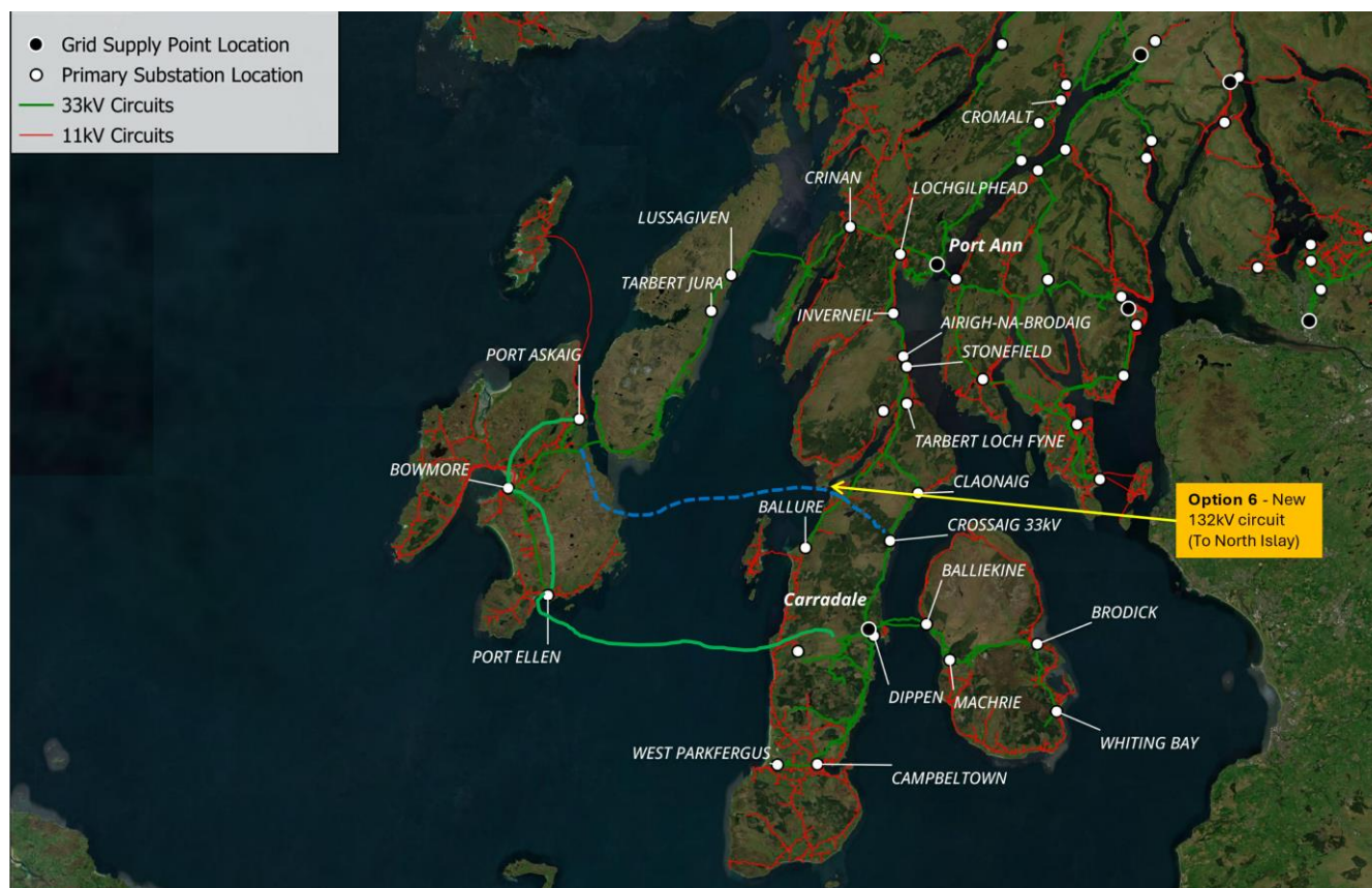
Figure 35 GIS view of network with works in progress and additional reinforcement options by 2040 (Option 6)
