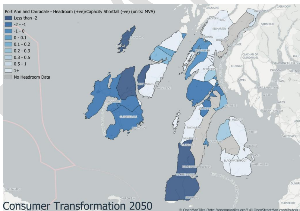
Figure 3 Port Ann GSP 2050 EHV network spatial plan (CT scenario)
