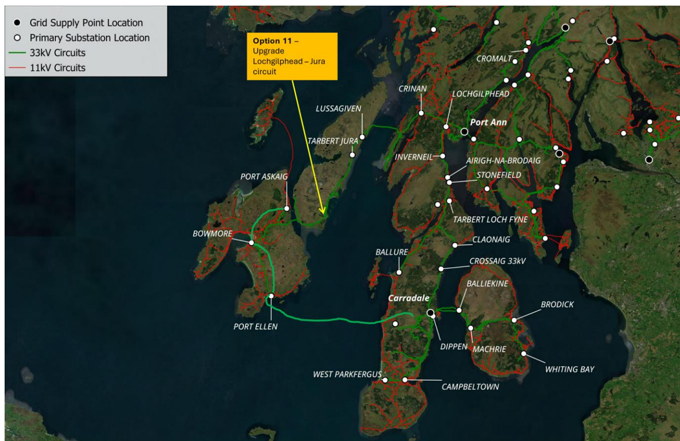
Figure 40 GIS view of network with works in progress and additional reinforcement options between 2041-2050 (Option 11)
