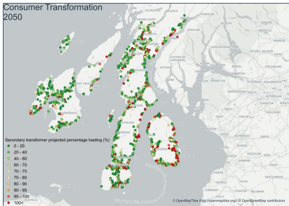
Figure 4 Port Ann and Carradale GSPs 2050 HV/LV network spatial plan CT Scenario
