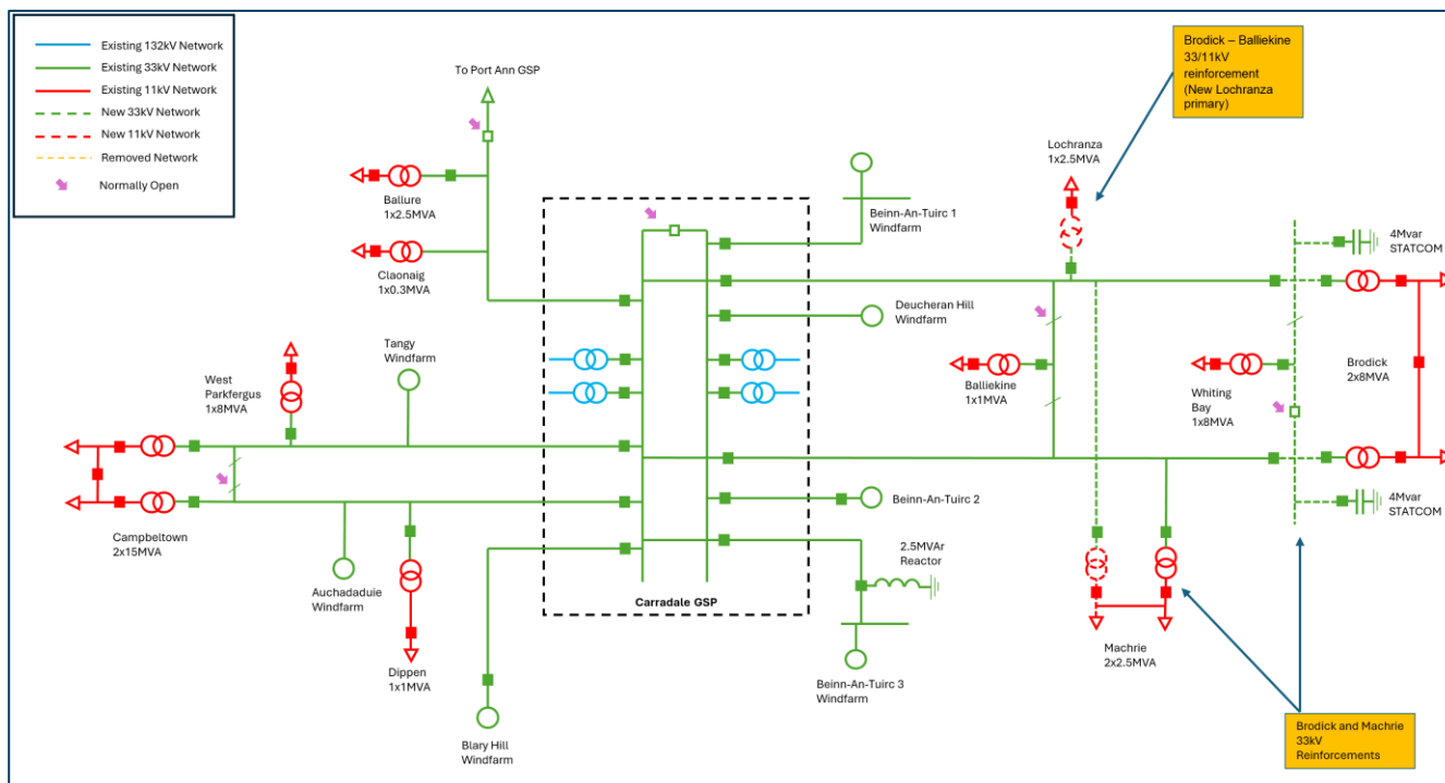
Figure 21 Future Network Development around Carradale GSP
