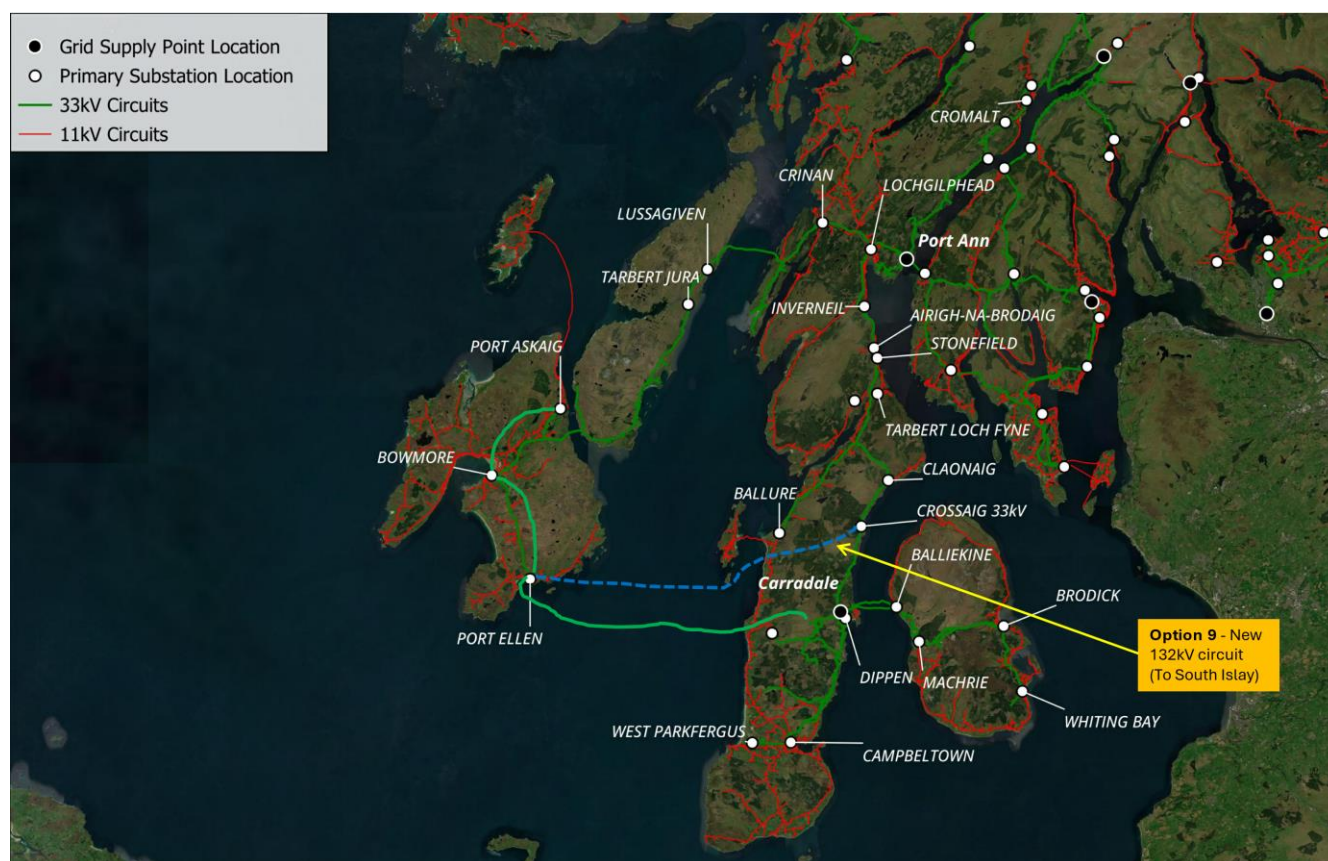
Figure 38 GIS view of network with works in progress and additional reinforcement options by 2040 (Option 9)
